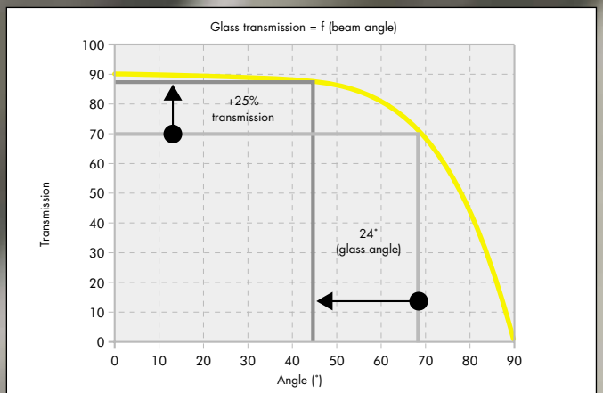
Champion's innovative optic gives improved output efficiency
